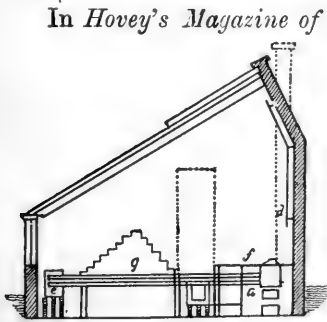
FIG. 3. MODEL GREENHOUSE OF 1835.
